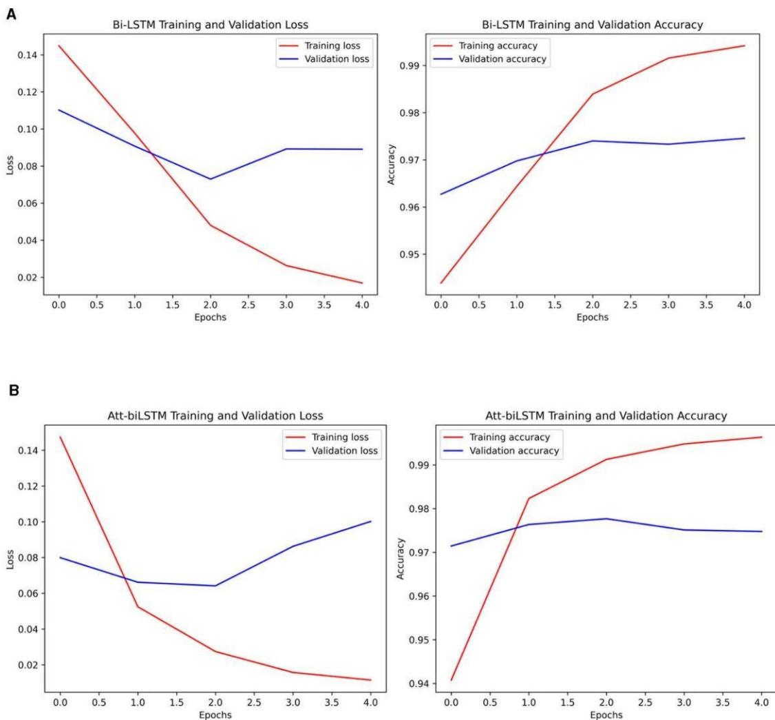
FIGURE 11 (A) BiLSTM and (B) Attention-based BiLSTM model loss and accuracy dynamics.
