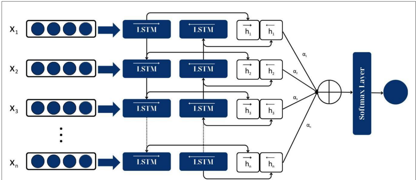
FIGURE 8 Attention-based BiLSTM model architecture.
