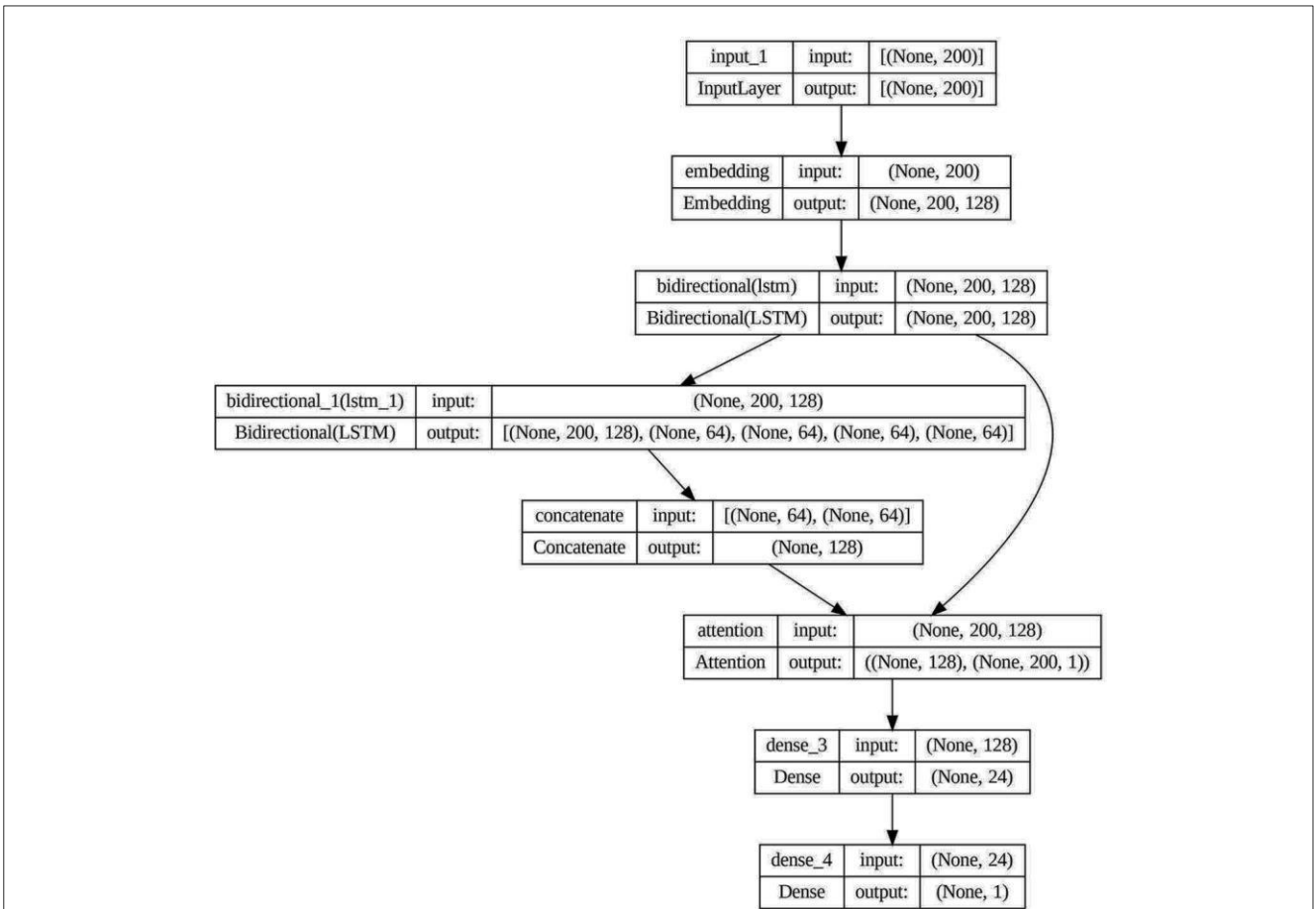
FIGURE 9 Architecture of proposed attention-based BiLSTM model.
