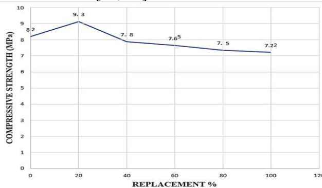
Figure 1: Compressive strength vs percentage replacement
