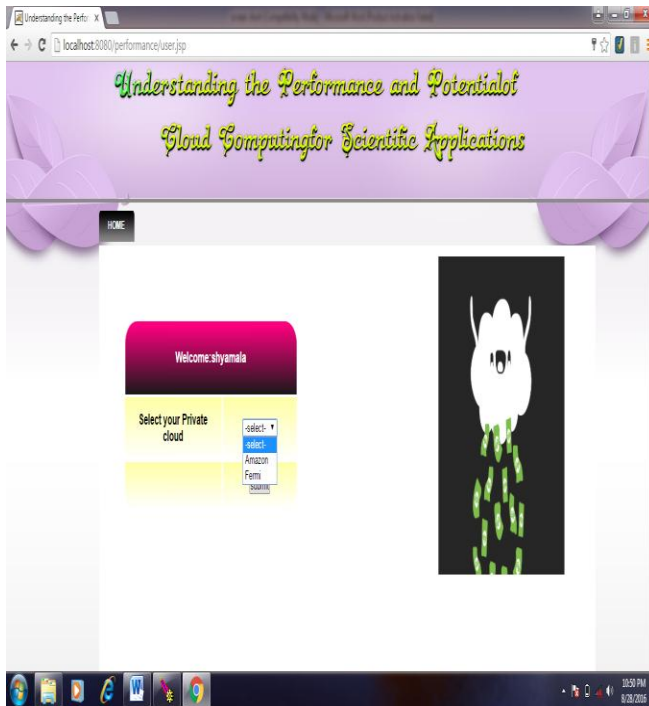
Fig 6.4: User Page
