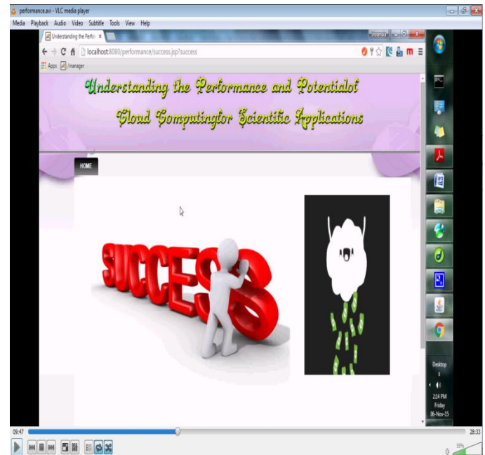
Success Page:
