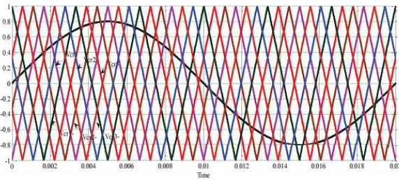
Fig. 2. Phase shift PWM for seven-level inverter
