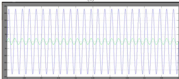
Fig. 6.(a) Five level Output voltage of inverter (b) In phase waveform of grid voltage and grid current (c) Harmonic Analysis of Grid Current
