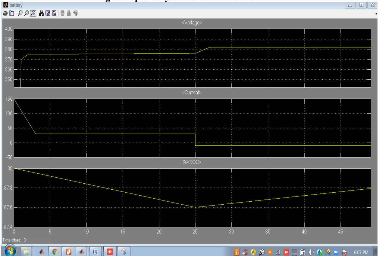
Fig 9 Battery voltage, current and SOC
