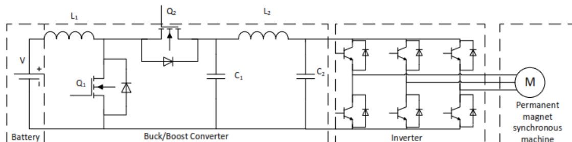
Fig 2 Proposed circuit configuration
