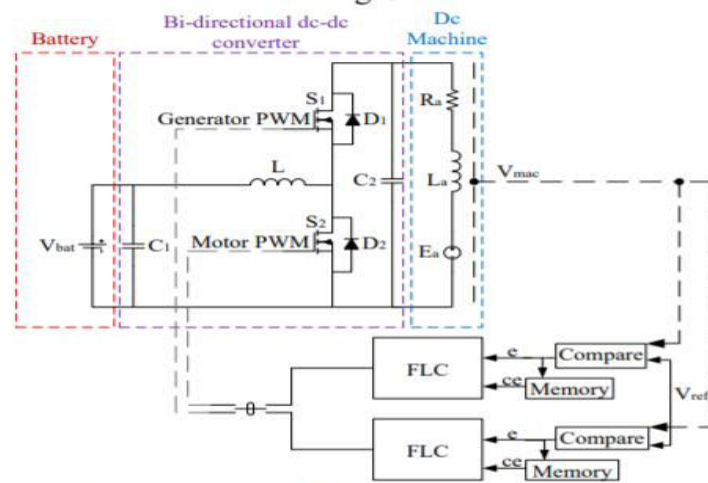
Fig 1 conventional circuit configuration
