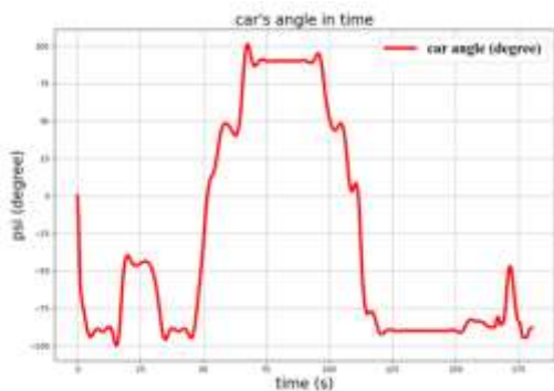
Yaw angle vs Time
