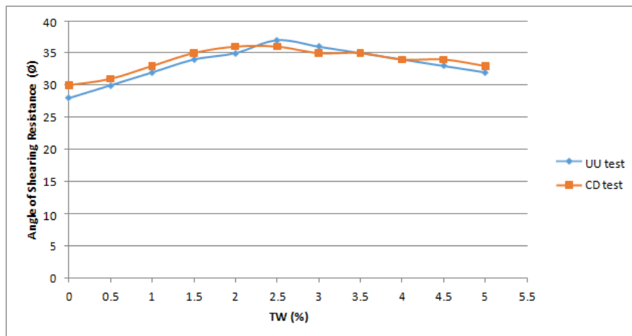
Graph.6: Variation of Angle of Shearing resistance ( \phi ) with percentage of TW
