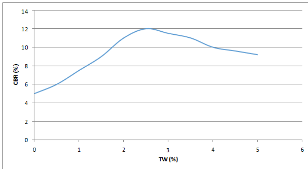
Graph.5: Variation of CBR (%) with percentage of TW
