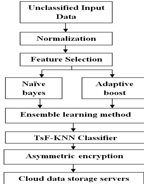
Fig. 1: SECURE MOBILE CLOUD COMPUTING SYSTEM USING ML CLASSIFICATION
