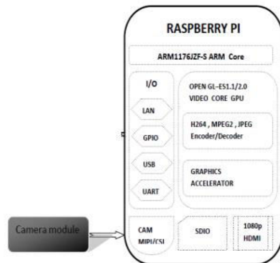
Figure 1 Block Diagram
