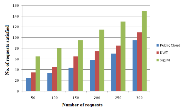
Figure 4: Dynamic resource management with time series in distributed cloud load balancing.
