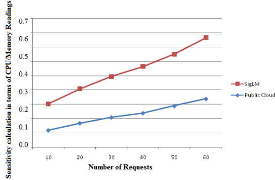
Figure 5: CPU/Memory readings in public distributed data.
