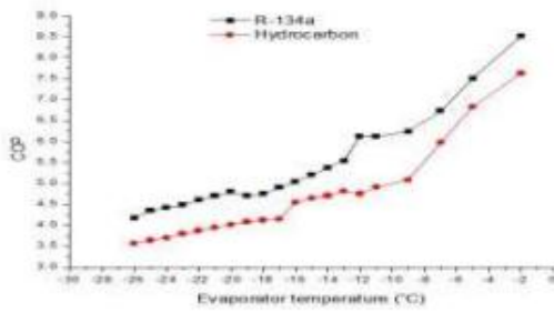
Fig. 8: Variation of COP with Evaporator Temperature
