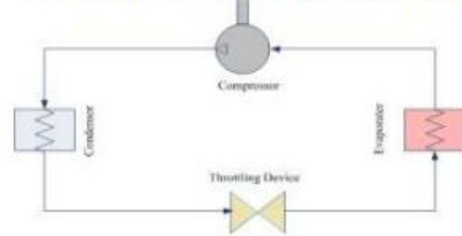
Fig. 4: Schematic diagram of Vapour compression refrigeration System
