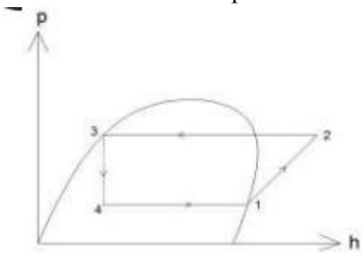
Fig. 1: p-h diagram of refrigeration cycle
