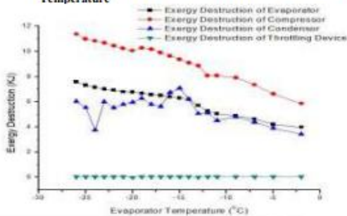
Fig. 10. Using R-134a Variation of ED with Evaporator Temperature
