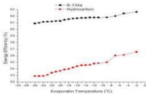
Fig. 9: Variation of Exergy Efficiency with Evaporator Temperature
