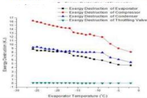
Fig. 11. Using Hydrocarbon Variation of ED with Evaporator Temperature
