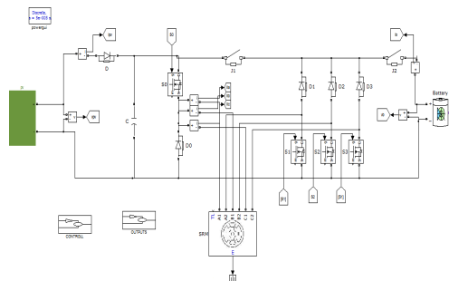
Fig 2 Existing circuit configuration
