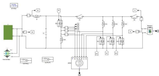
Fig 2 Existing circuit configuration
