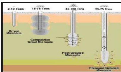
Figure No. 6Micro Pile Foundations with Micro Piles
