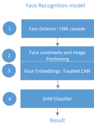
Fig. 4. Face Recognition Model.
