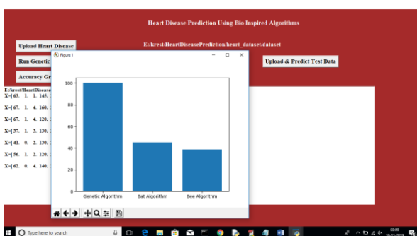
Fig.5. Accuracy Graph.
