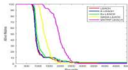
Figure 4 Plot of comparison of network lifetime LEACH, LEACH-E, LEACH-EX, GADA-LEACH and MHTRP-LEACH at E_o=0.4J
