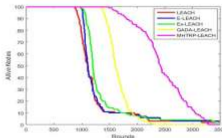
Figure 7 Plot of comparison of network lifetime LEACH, LEACH-E, LEACH-EX GADA-LEACH and MHTRP-LEACH when packet size=2000
