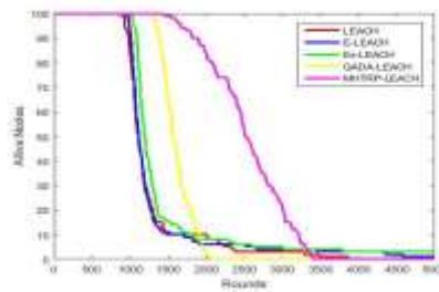
Figure 5 Plot of comparison of network lifetime LEACH, LEACH-E, LEACH-EX, GADA-LEACH and MHTRP-LEACH at E_o = 0.5J/node
