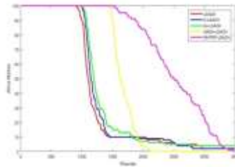
Figure 8 Plot of comparison of network lifetime LEACH, LEACH-E, LEACH-EX, GADA-LEACH and MHTRP-LEACH when packet size=3000
