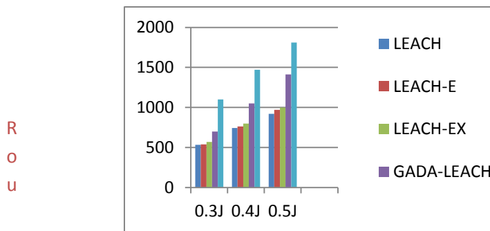
Figure 6 Network Lifetime of LEACH, LEACH-E, LEACH-EX GADA-LEACH and MHTRP-LEACH when varying E_o
