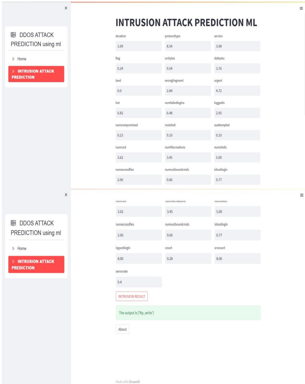
Fig 2: Expected Output
