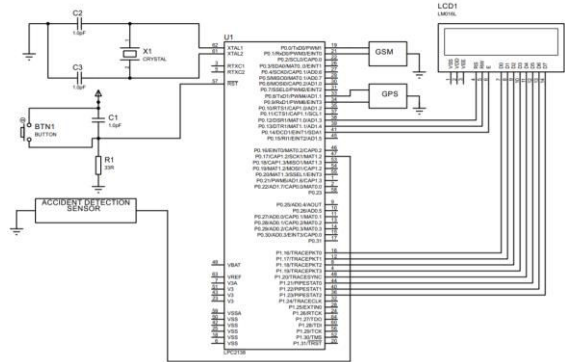
Fig. 5: WHEN ACCIDENT DETECTION SENSOR IS DETECTED
