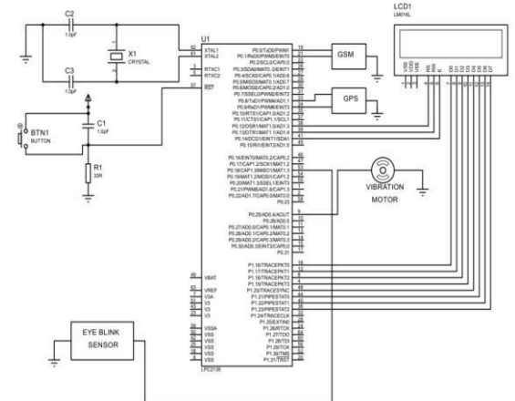
Fig. 6: WHEN EYE BLINK SENSOR IS ACTIVATED
