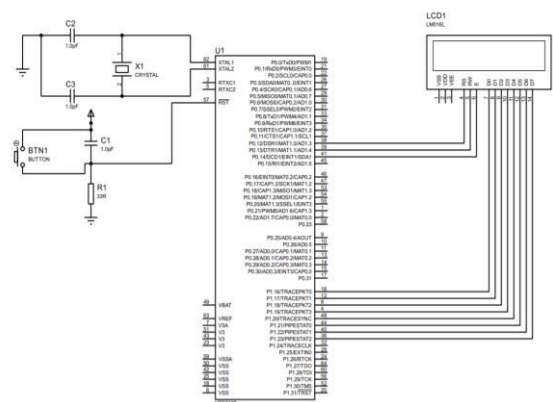
Fig. 2: BASIC CIRCUIT DIAGRAM
