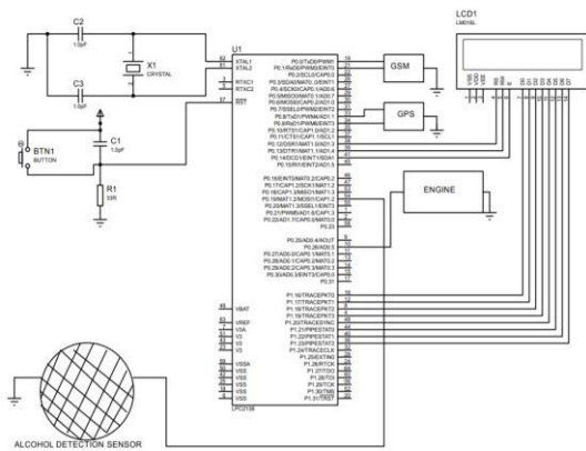
Fig. 4: WHEN ALCOHOL DETECTION SENSOR IS ACTIVATED
