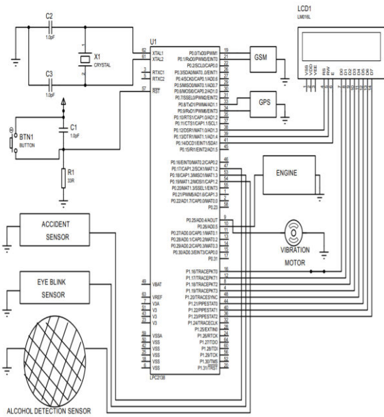
Fig. 3: CIRCUIT DIAGRAM OF PROPOSED SYSTEM
