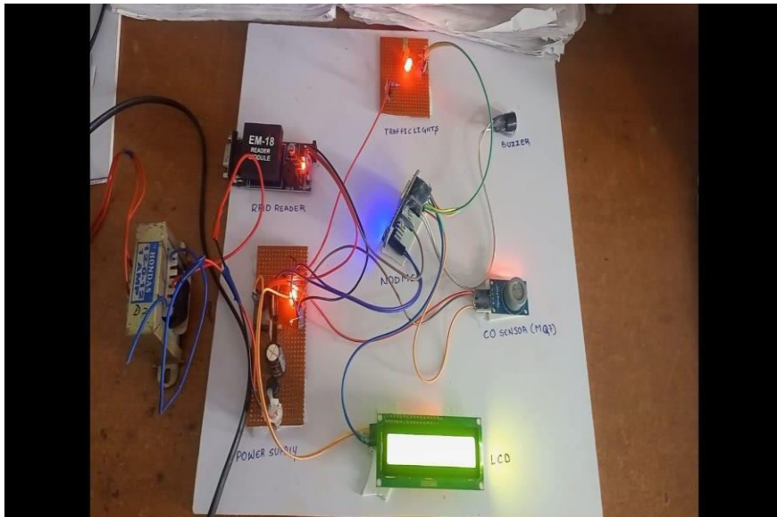
Figure.6 Working Kit
