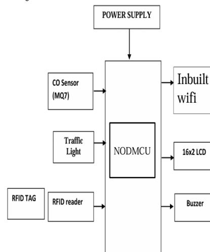
Figure.1 Block Diagram
