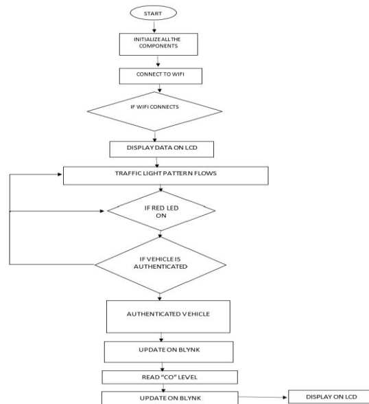
Figure.3 Flow Chart
