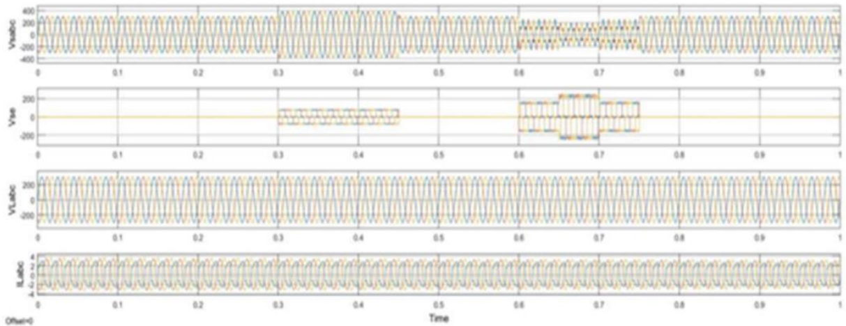
Fig2. Three phase Load Current and Load Voltage
