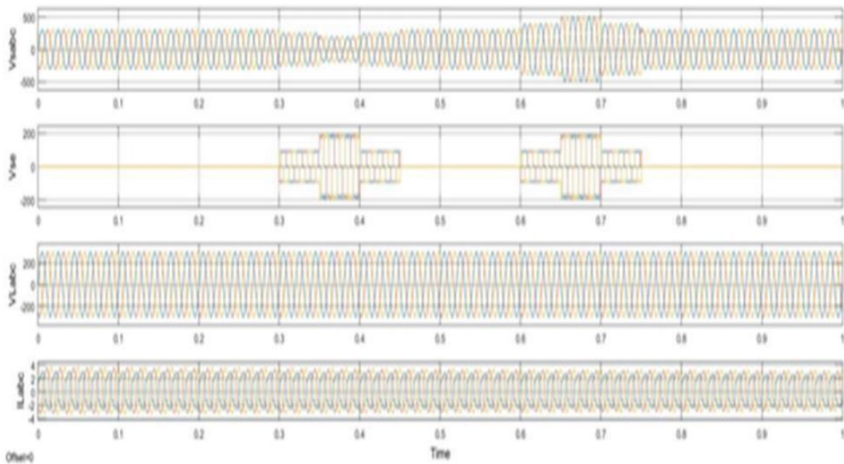
Fig 8. Load currents and load voltages
