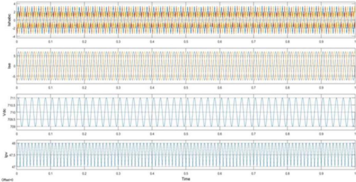
Fig 7. PV currents and DC voltages
