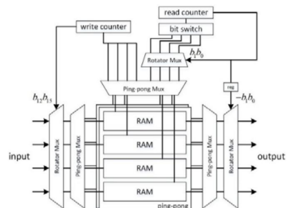
Fig. 1: FFT PROCESSOR
