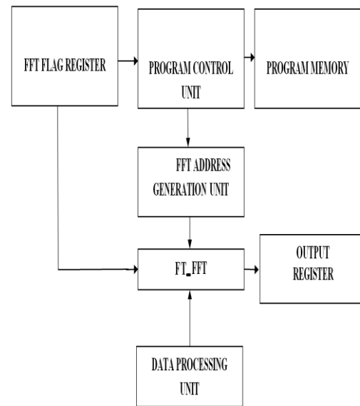
Fig. 2: PROPOSED SYSTEM
