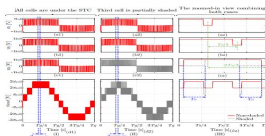
Fig. 2 The resulting voltage for all power cells case the came about absolute result voltage, in the twocases,
