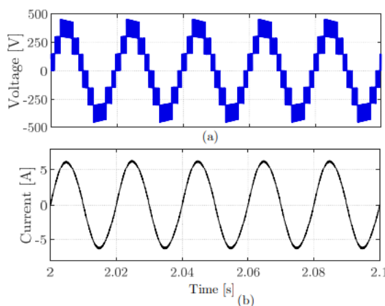
Fig. 7 (a) The outcome voltage, (b) the affiliation current, when the three PV strings of the proposed topography are under the standard test conditions
