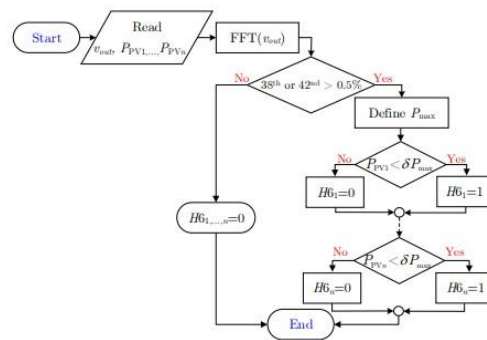
Fig. 5 Flowchart of Algorithm Used to Determine Partially Shaded Power Cells
